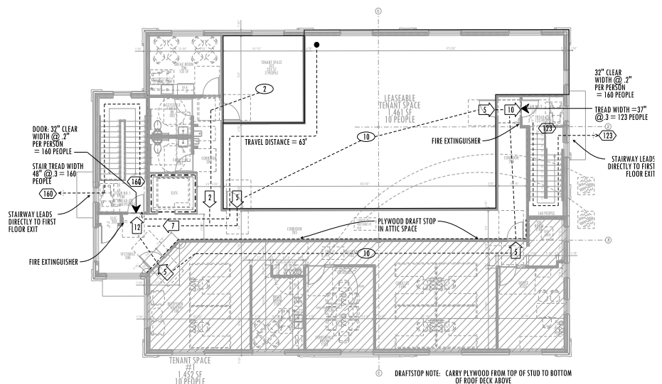
Floor Plan - 2nd Floor
