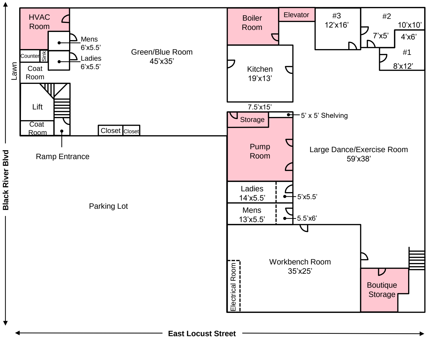
Floor Plan
