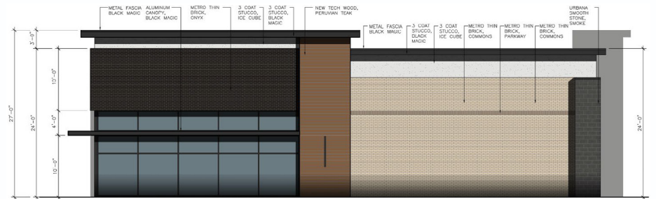
EAST FACING ELEVATION
